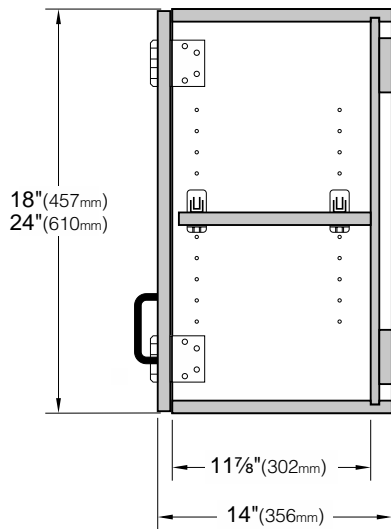
18" & 24" High Wall Cabinets
