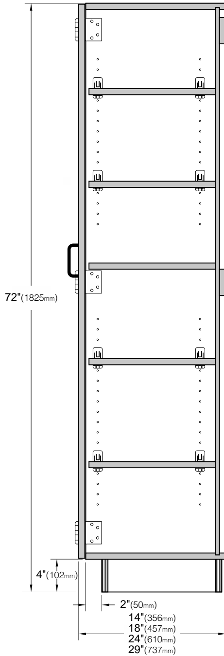
72" High Tall Cabinets
