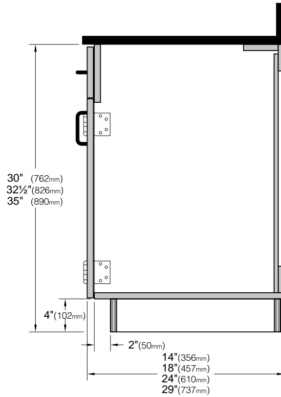
Sink Cabinet
