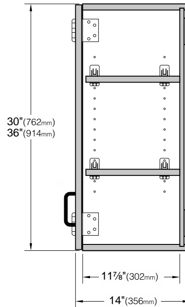
30" & 36" High Wall Cabinets
