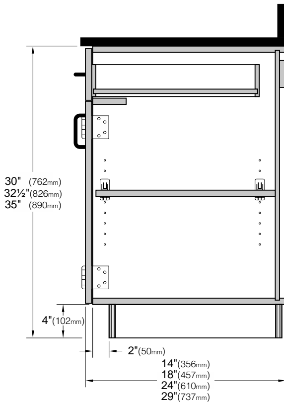
Base Cabinet
