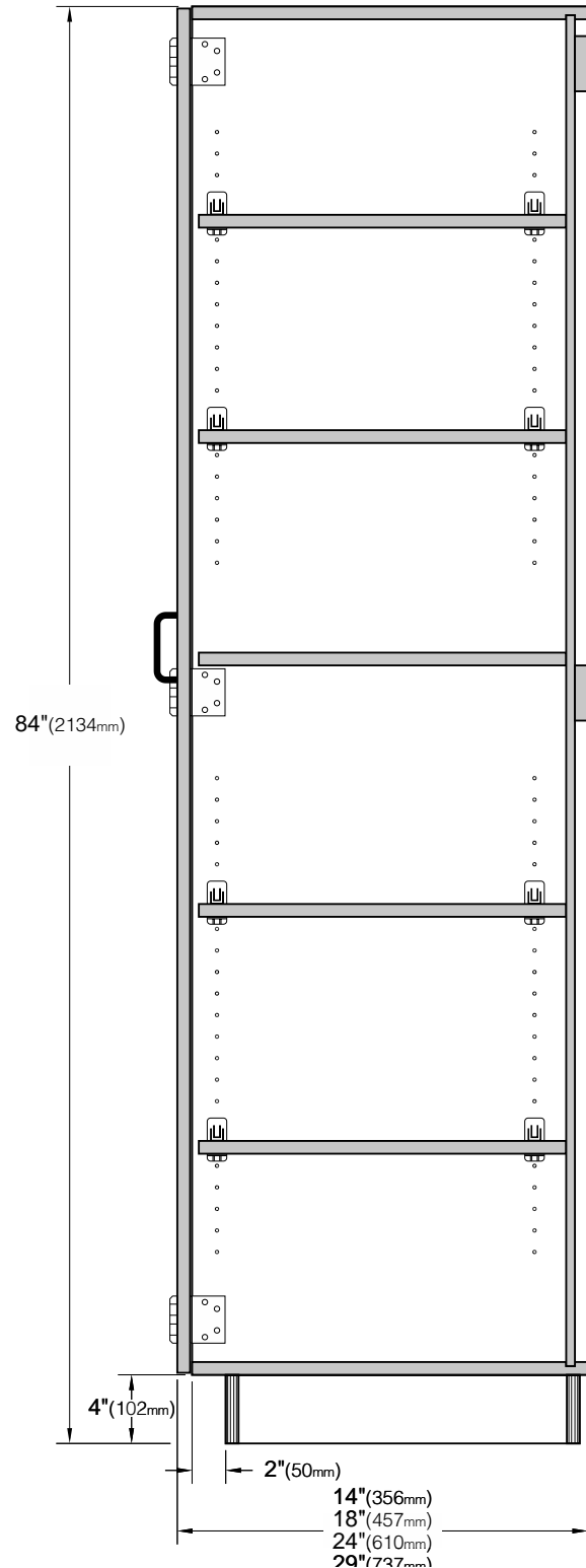
84" High Tall Cabinets
